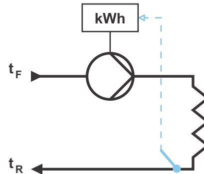
Fig. 28 MAGNA3 with built-in heat energy meter
