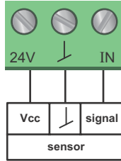
Fig. 40 Analog input for external sensor or control
