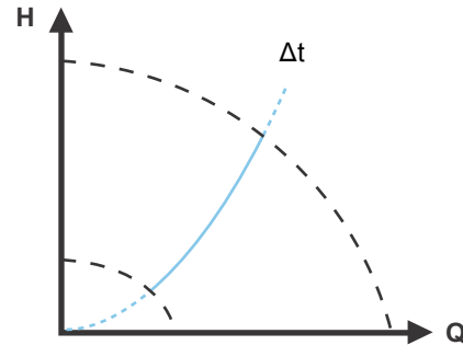
Fig. 16 Differential-temperature control
