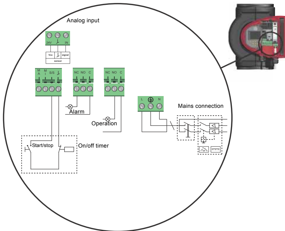
Fig. 37 Example of connections in the control box
