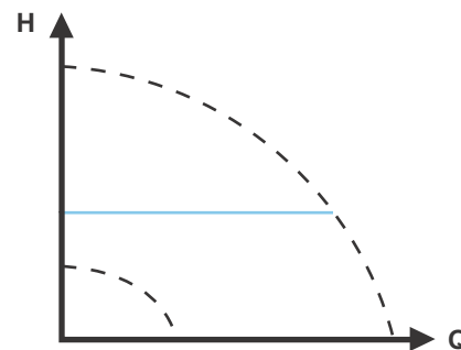
Fig. 12 Constant-pressure control
