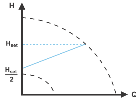
Fig. 11 Proportional-pressure control
