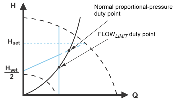
Fig. 20 Proportional-pressure control with FLOW LIMIT
