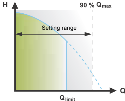
Fig. 19 FLOW LIMIT
