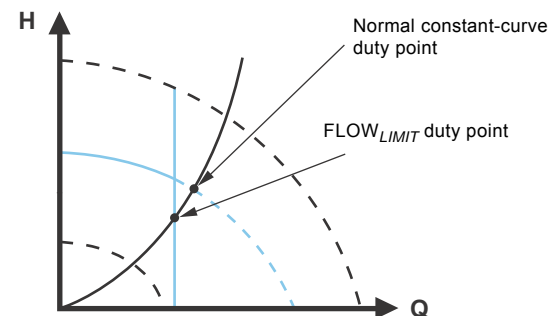
Fig. 22 Constant curve with FLOW LIMIT
