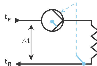
Fig. 17 Pump with external sensor
