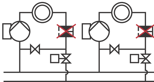
Fig. 9 Reduced need for a pump throttling valve
