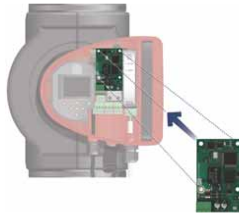
Fig. 45 Location of CIM module
