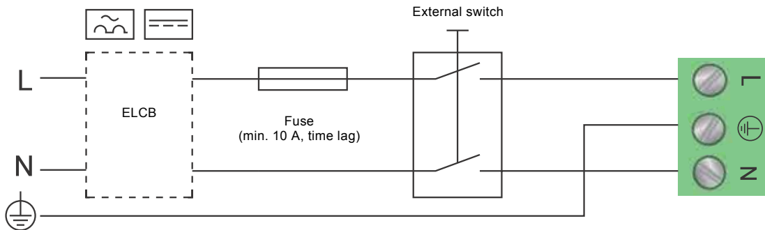
Fig. 36 Example of typical connection, 1 x 230 V ± 10 %, 50/60 Hz
