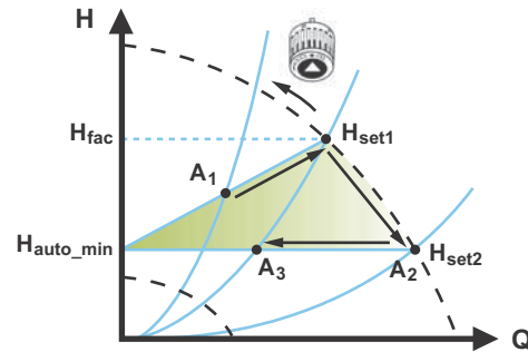
Fig. 8 AUTO_{ADAPT} control
