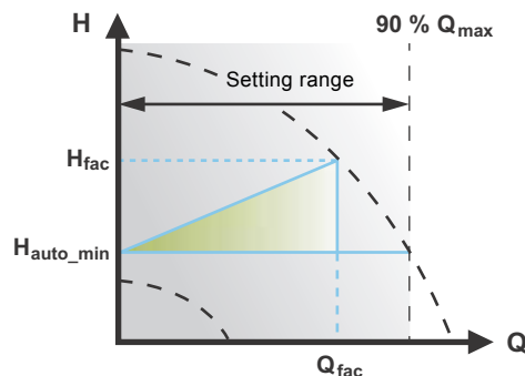
Fig. 10 FLOW ADAPT control
