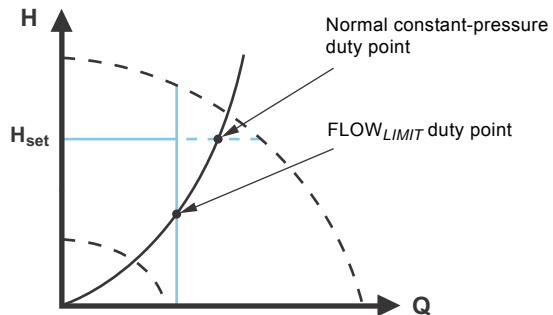
Fig. 21 Constant-pressure control with FLOW LIMIT
