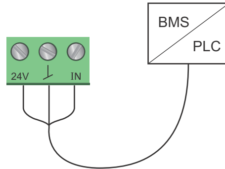
Fig. 43 Example of external signal for the control via BMS or PLC
