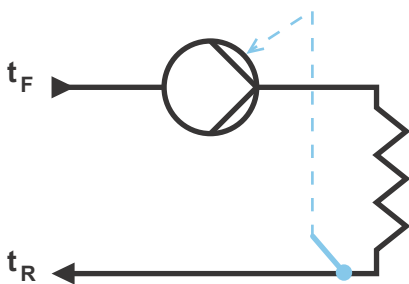
Fig. 15 Pump with external sensor
